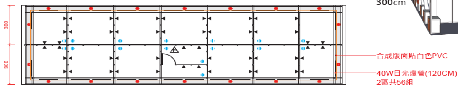
1/3 FLOOR PLAN S:1/100
